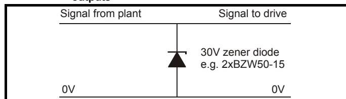
Figure 4-19 Surge suppression for analog and bipolar inputs and
