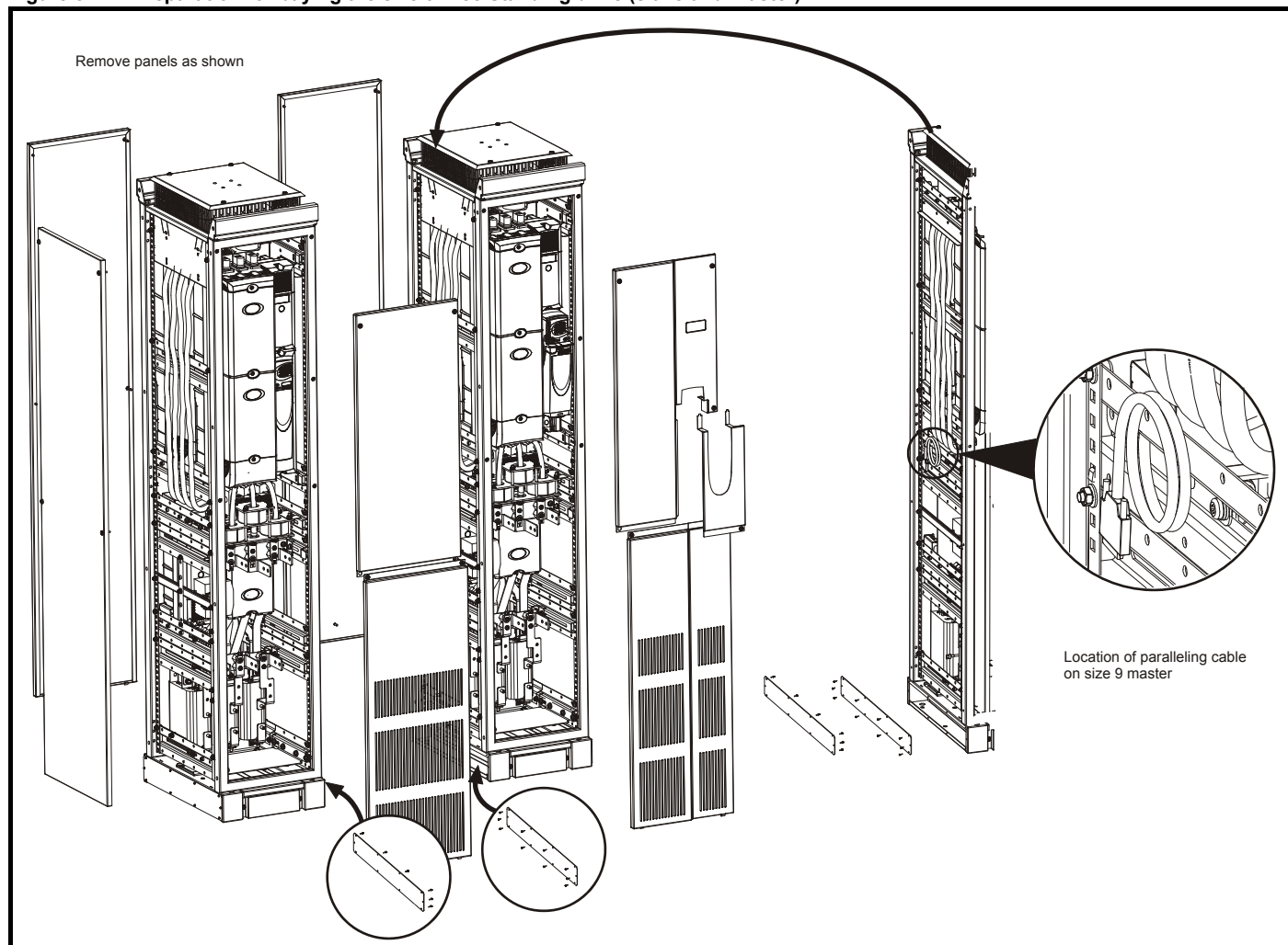
Figure 3-12 Preparation for baying the size 9 Free Standing drive (slave and master)
