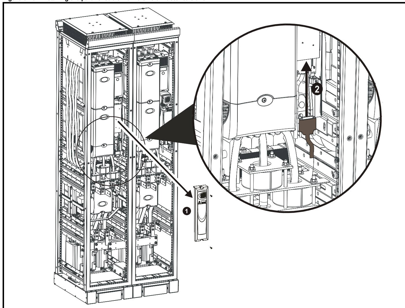
Figure 3-15 Installing the parallel cable from a size 9 master to slave
