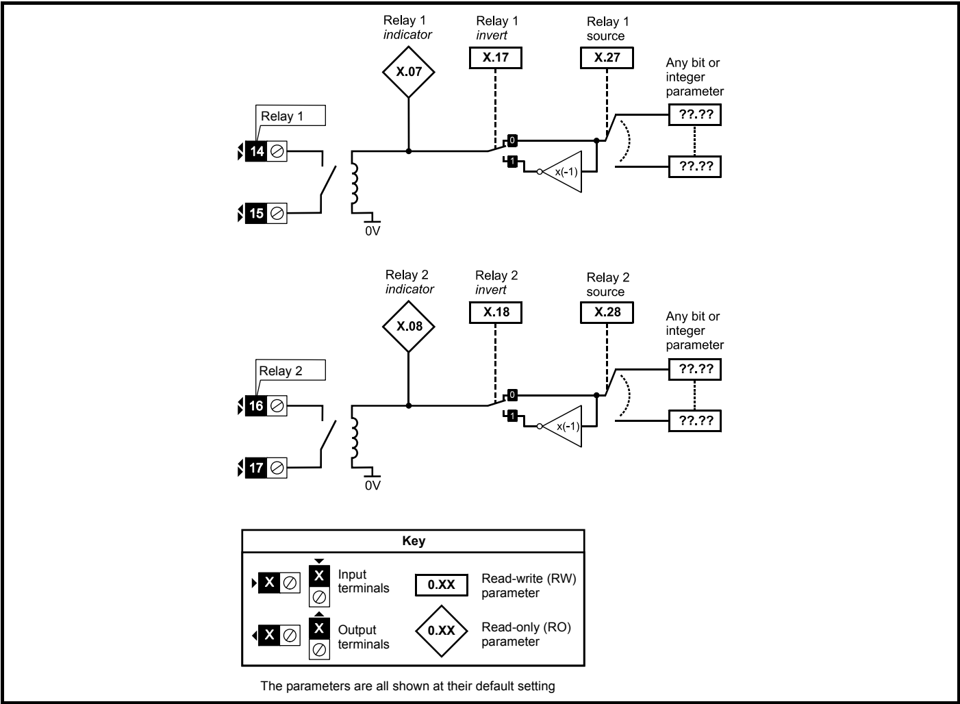
Figure 11-37 SM-I/O PELV relay logic diagram
