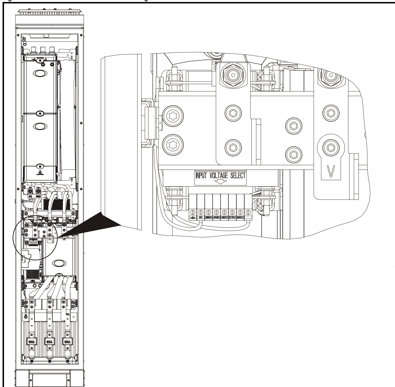
Figure 4-9 Location of size 8 and 9 Free Standing drive mains transformer
