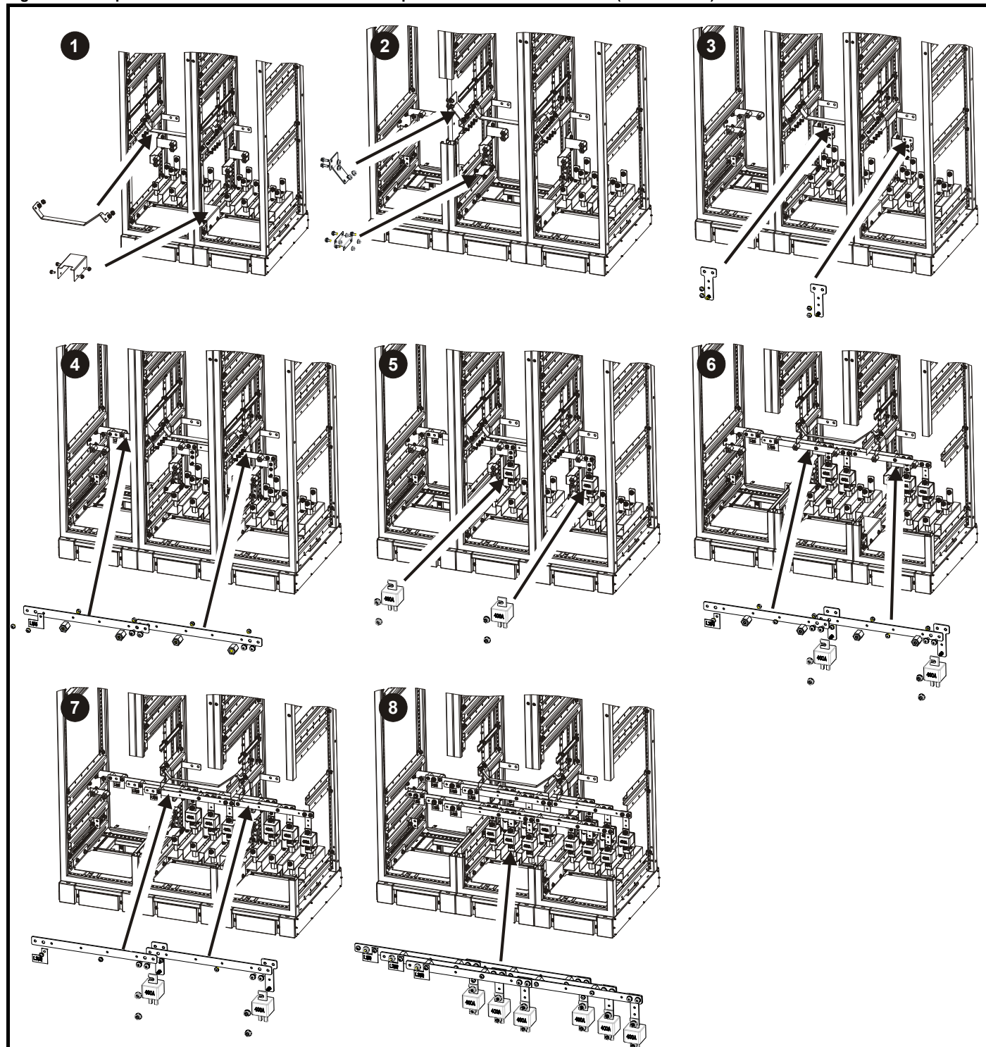
Figure 3-17 Input busbar connections between the 12 pulse size 9 master and slave (and incomer)
