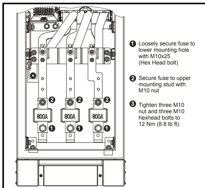
Figure 3-9 Installing DIN110 type fuses
