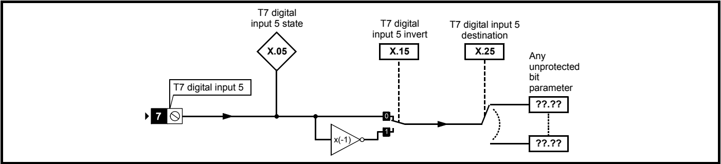
Figure 11-36 SM-I/O PELV digital input logic diagram
