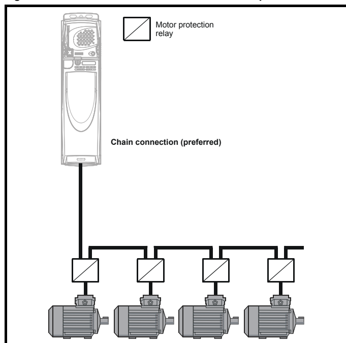
Figure 4-11 Preferred chain connection for multiple motors
