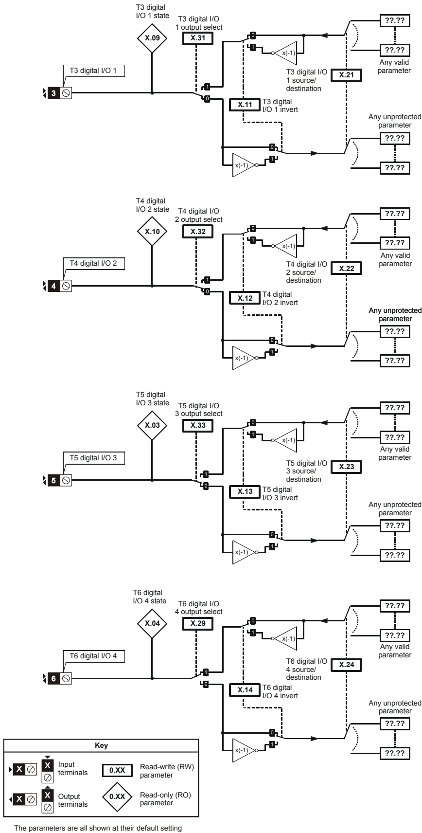
Figure 11-40 SM-I/O 24V Protected digital I/O logic diagram
