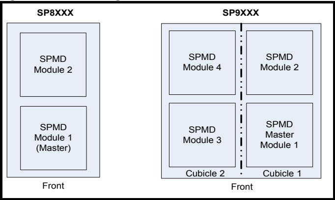
Figure 2-3 Drive configuration
