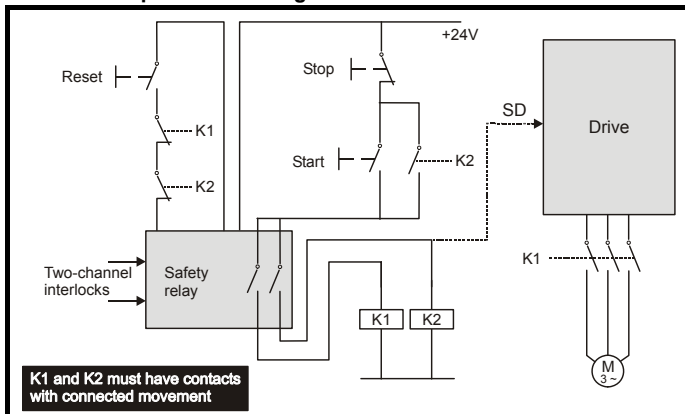
Figure 4-26 Use of contactor and relay to avoid the need for protected wiring
