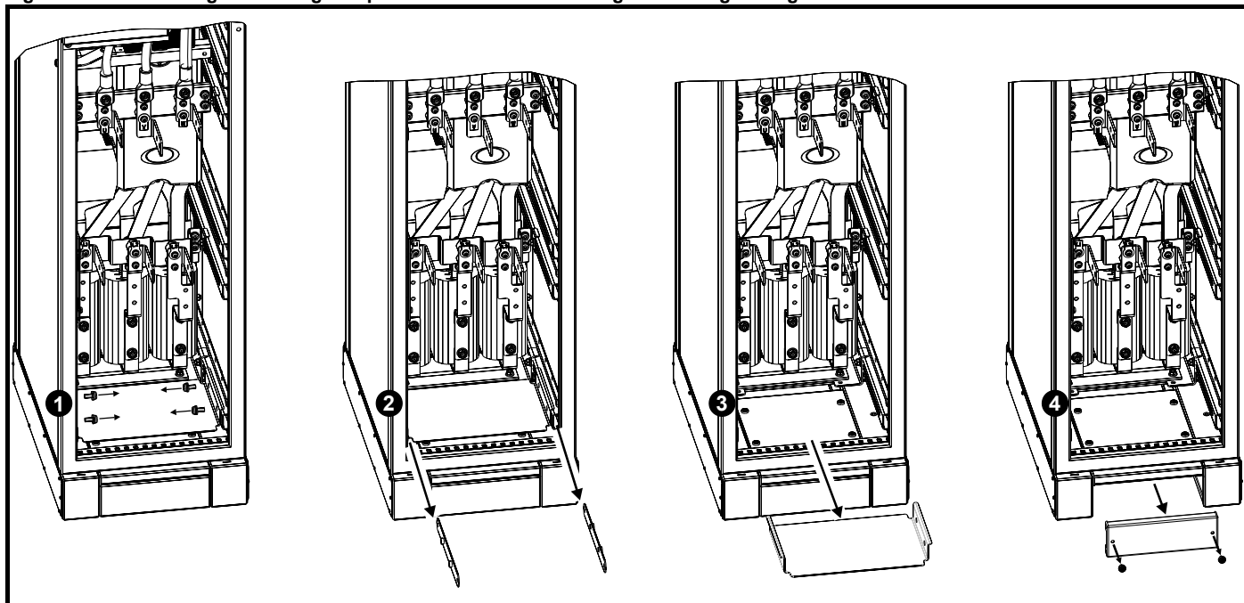
Figure 3-19 Removing the cable gland plate from the Free Standing drive for "glanding off" the cable
