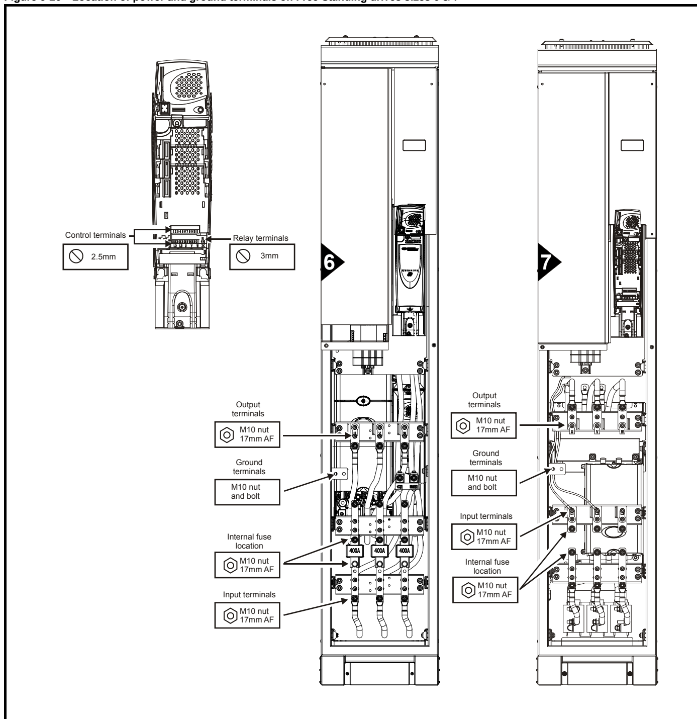
Figure 3-26 Location of power and ground terminals on Free Standing drives sizes 6 & 7
