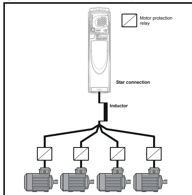
Figure 4-12 Alternative connection for multiple motors
