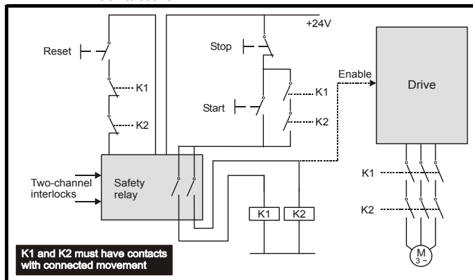
Figure 4-24 Category 3 interlock using electromechanical safety contactors
