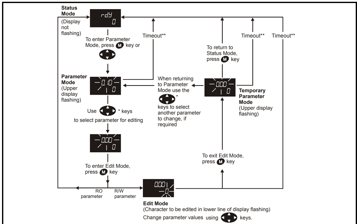
Figure 5-3 Display modes
