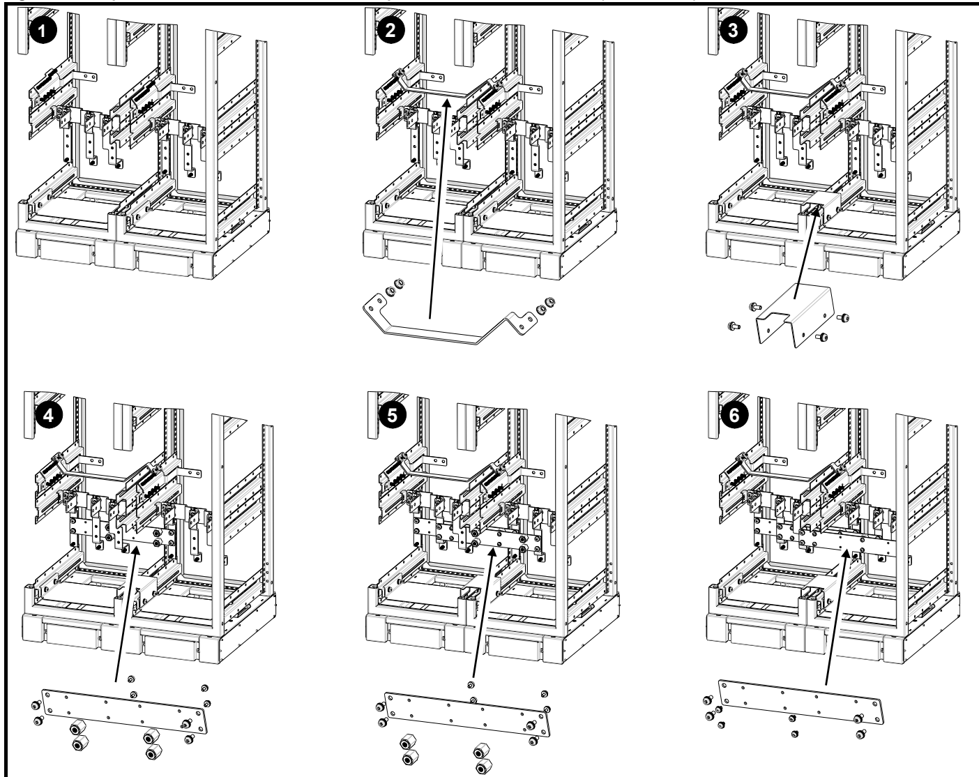
Figure 3-16 Input busbar connections between the 6 pulse size 9 master and slave (and incoer)
