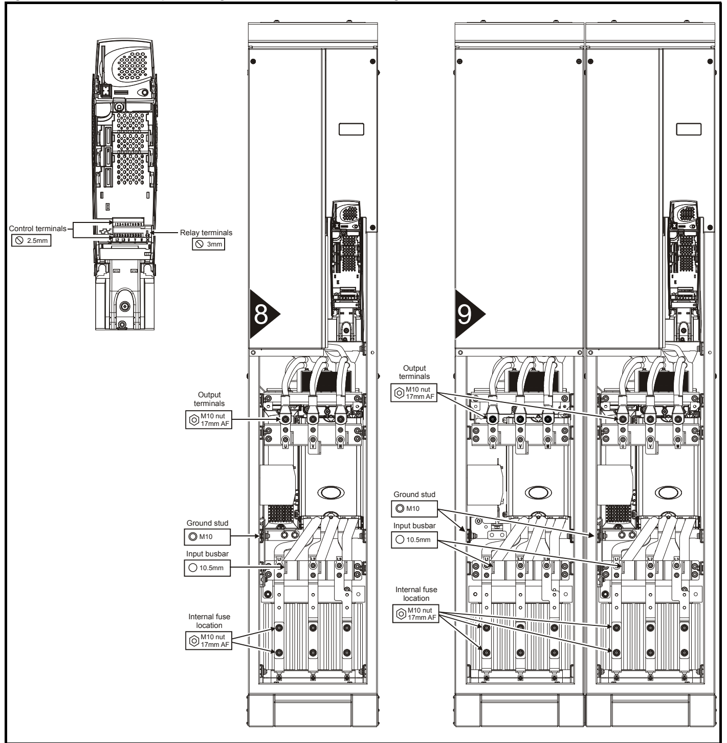
Figure 3-27 Locations of the power and ground terminals on Free Standing drives sizes 8 and 9
