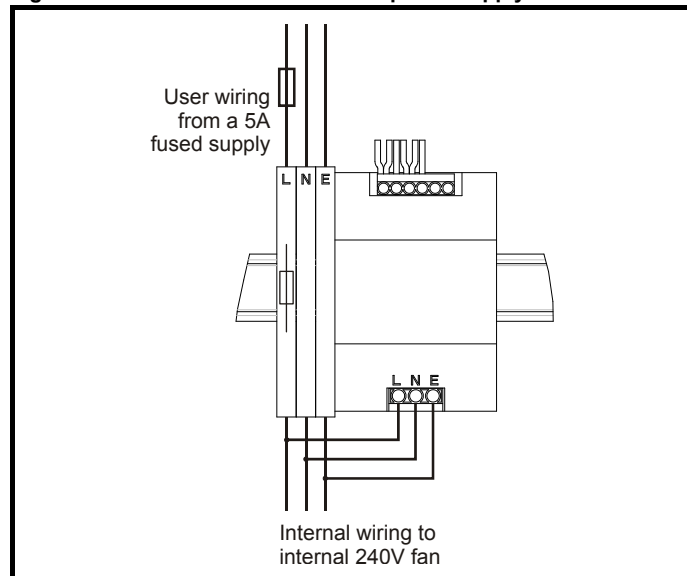
Figure 4-8 SP8XX4 and SP9XX5 24V power supply
