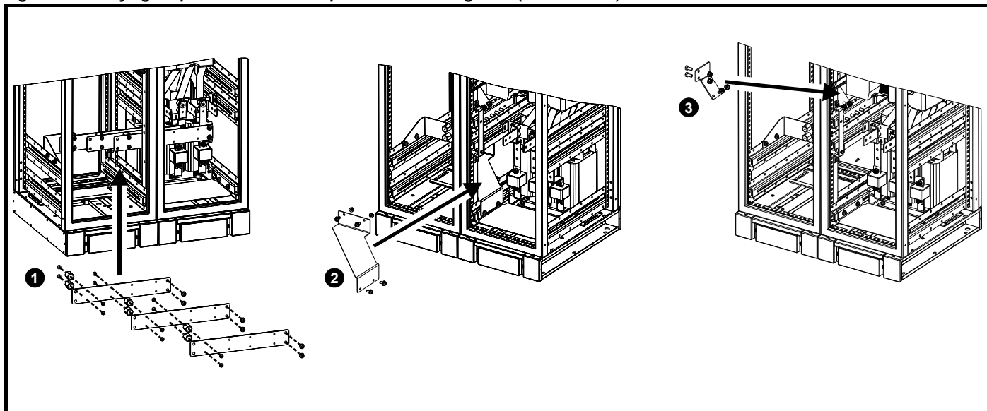
Figure 3-18 Baying a 6 pulse incomer to a 6 pulse Free Standing drive (size 8 shown)
