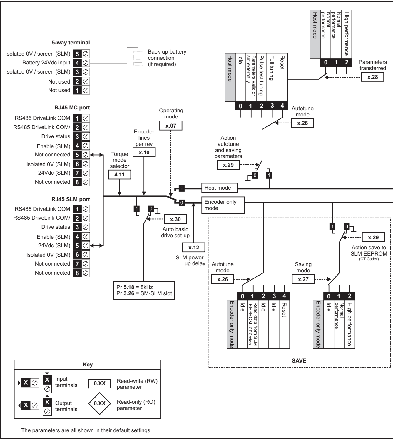
11.15.5 SLM module category Figure 11-46 SM-SLM logic diagram
