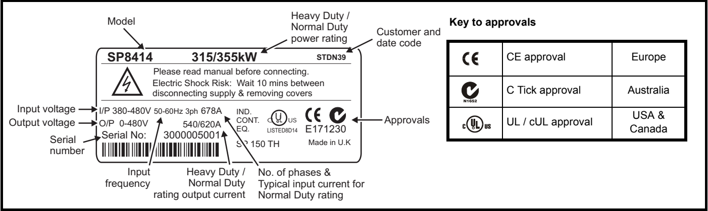
Figure 2-6 Typical drive rating label
